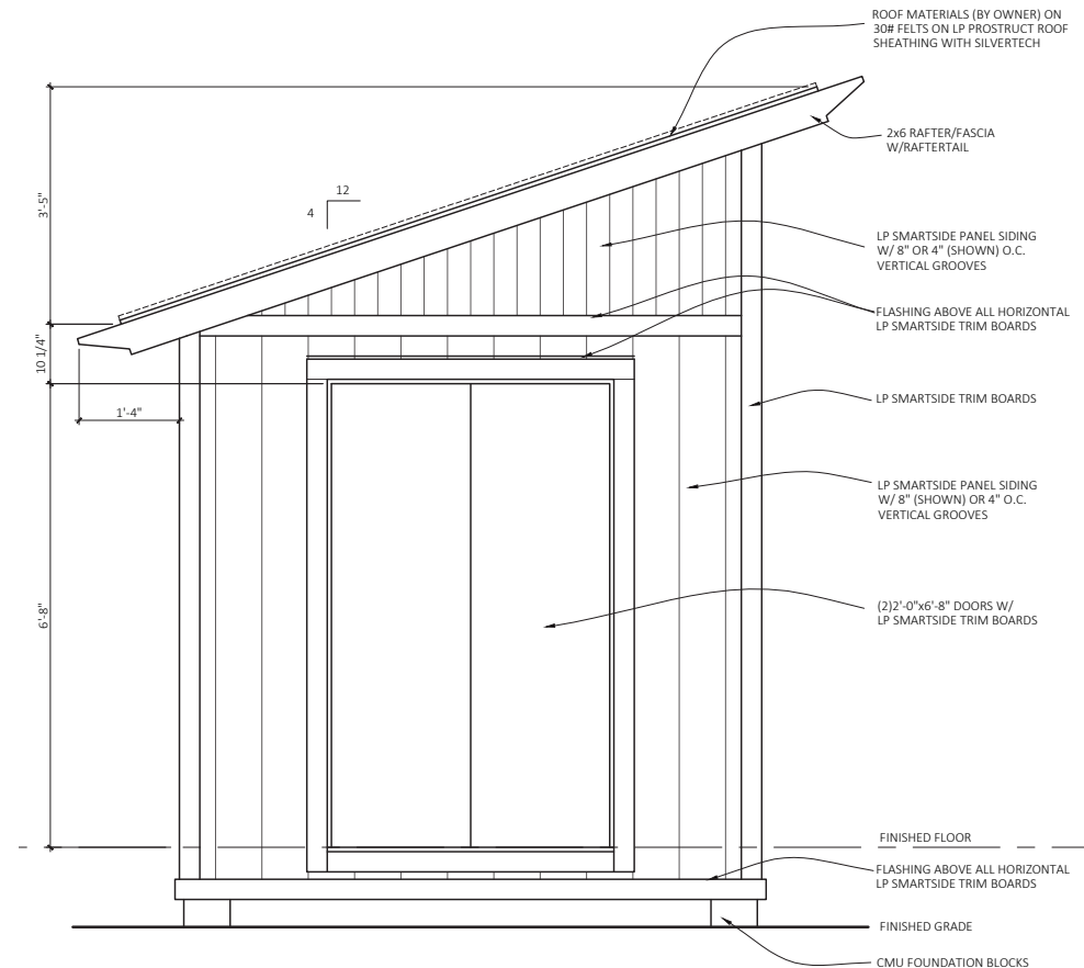
Front Elevation
