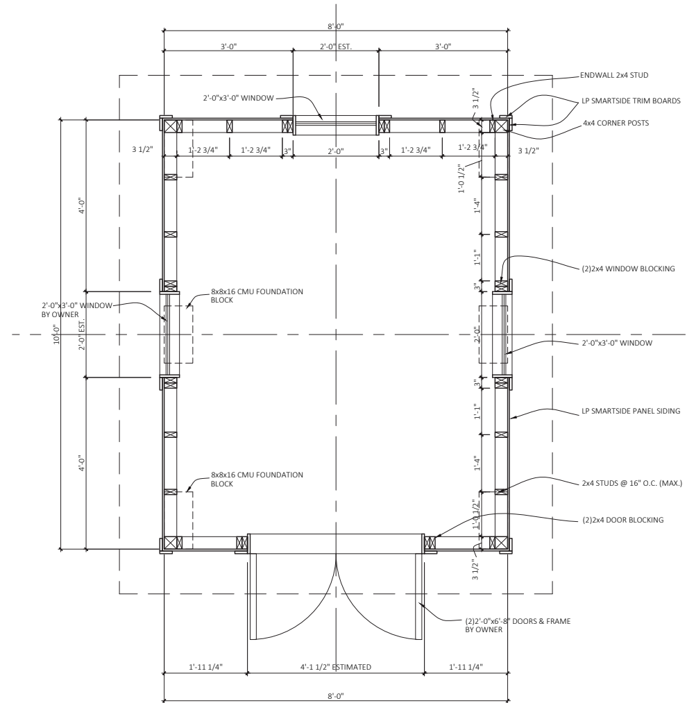
Floor Plan
