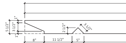
5 Roof Rafter Cuts
