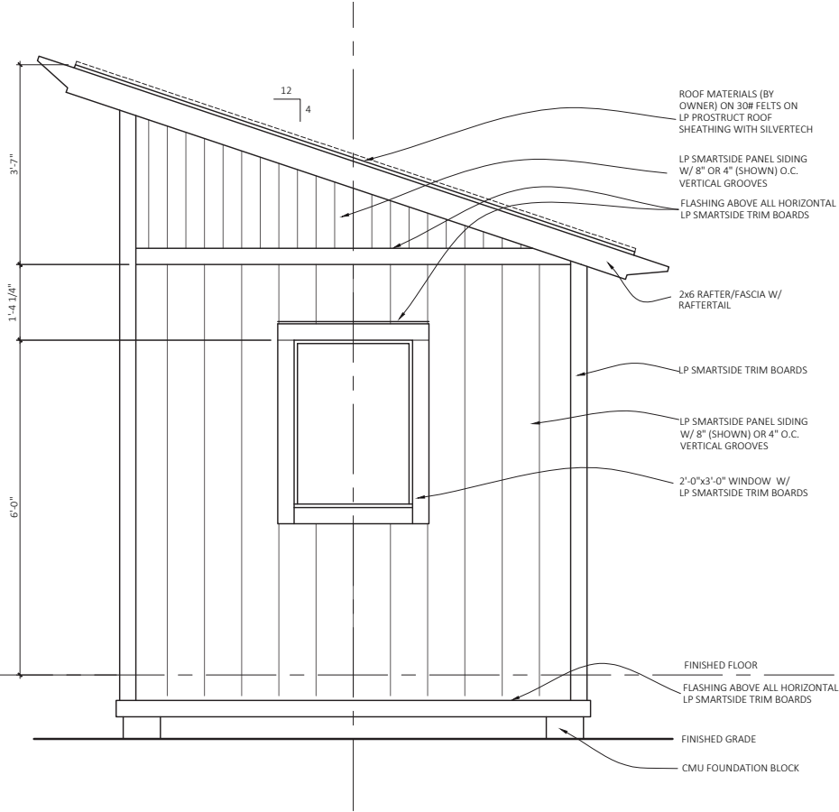
Rear Elevation
