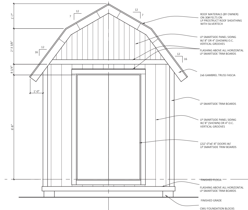
Front Elevation
