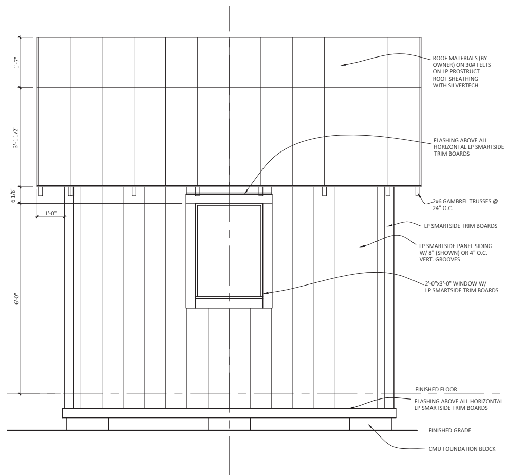
Left & Right Side Elevations
