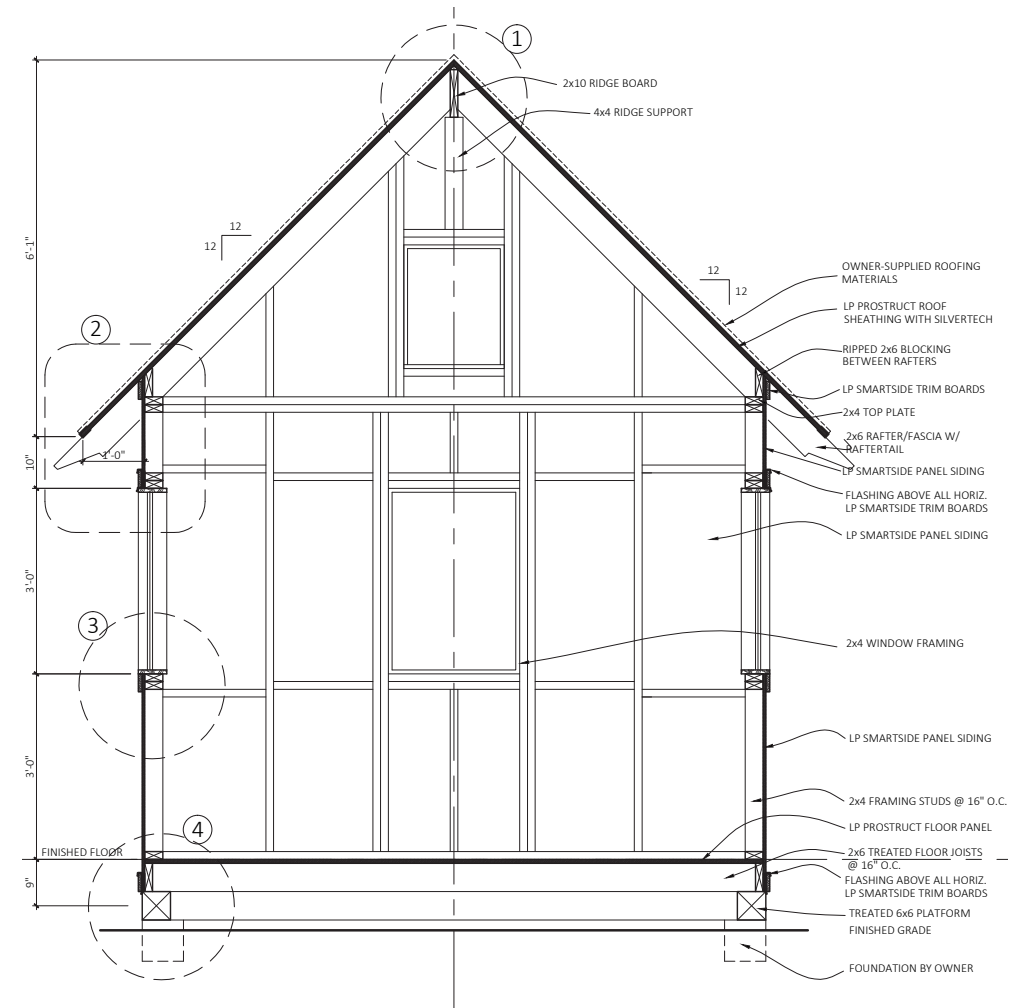
Cross-Section
