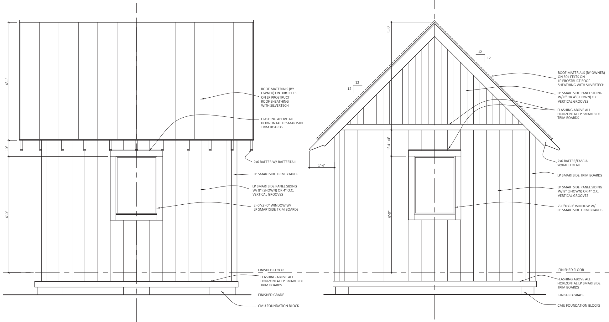
Left & Right Side Elevations
