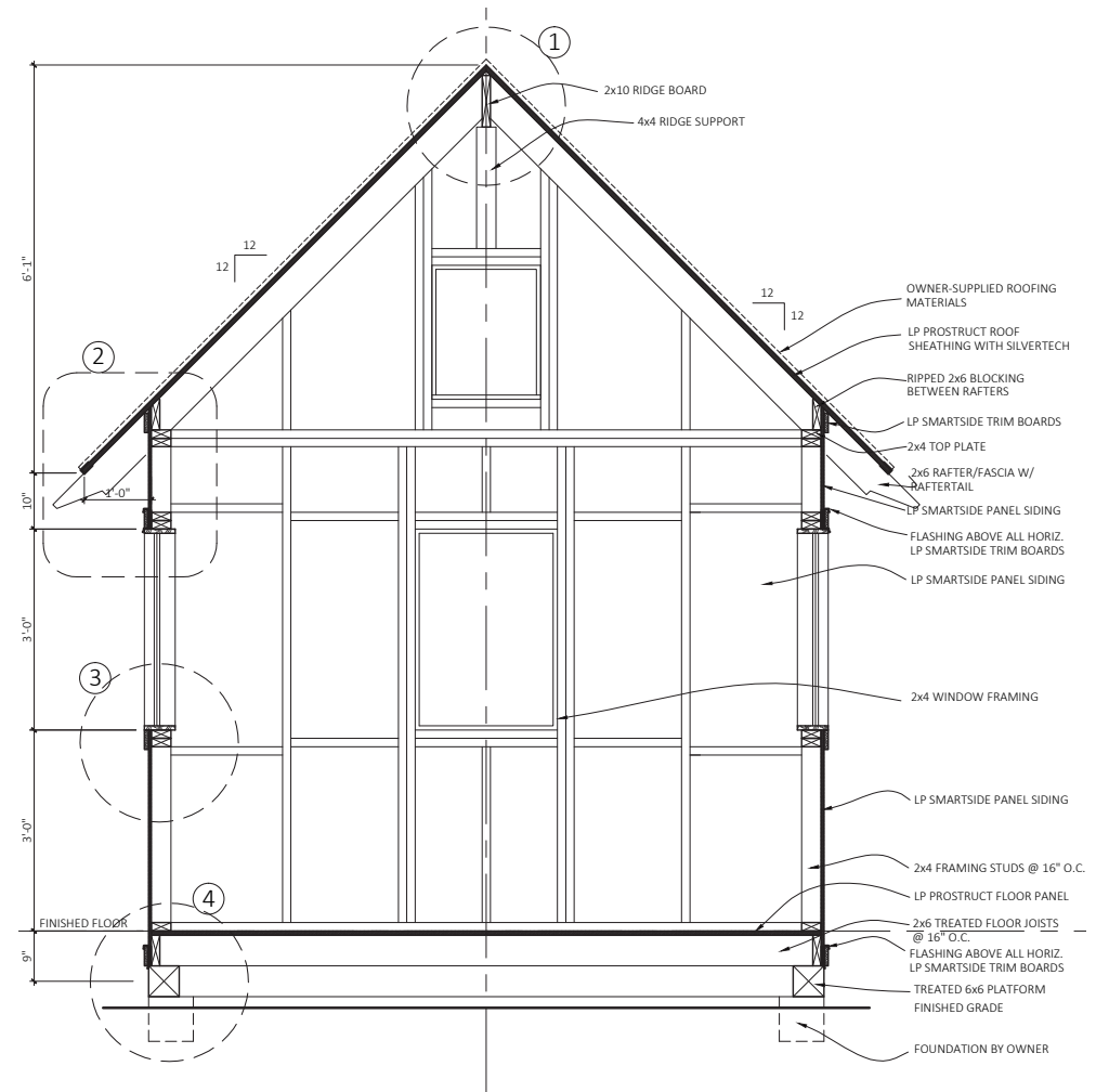
Cross-Section
