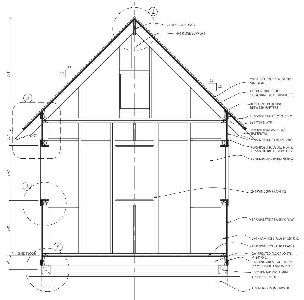
Cross-Section
