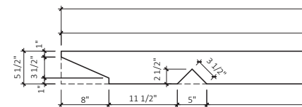
5 Roof Rafter Cuts
