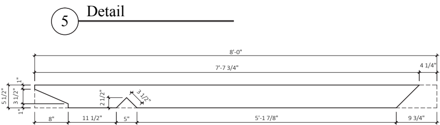
6 Roof Rafter Cuts
