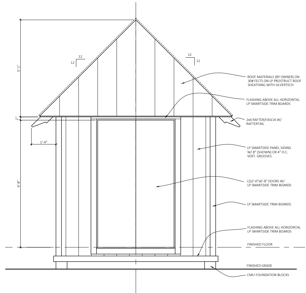
Front Elevation
