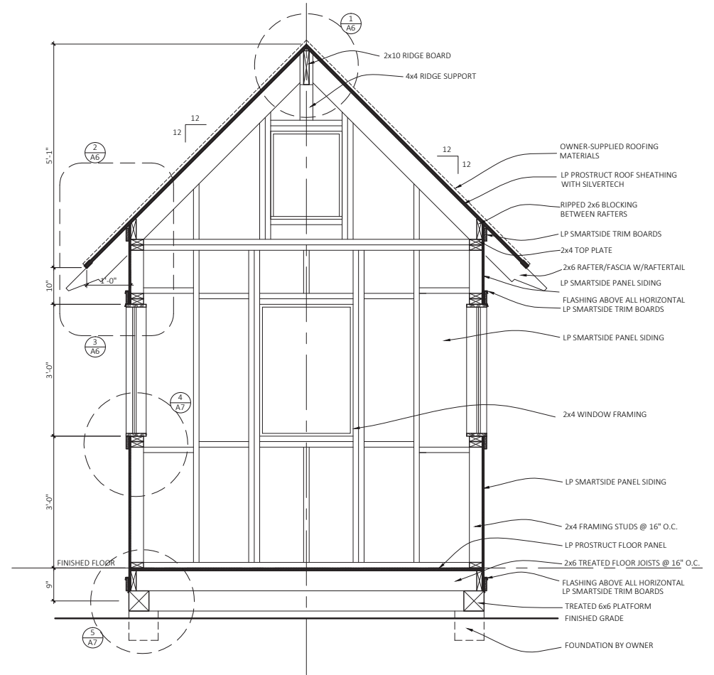
Cross-Section
