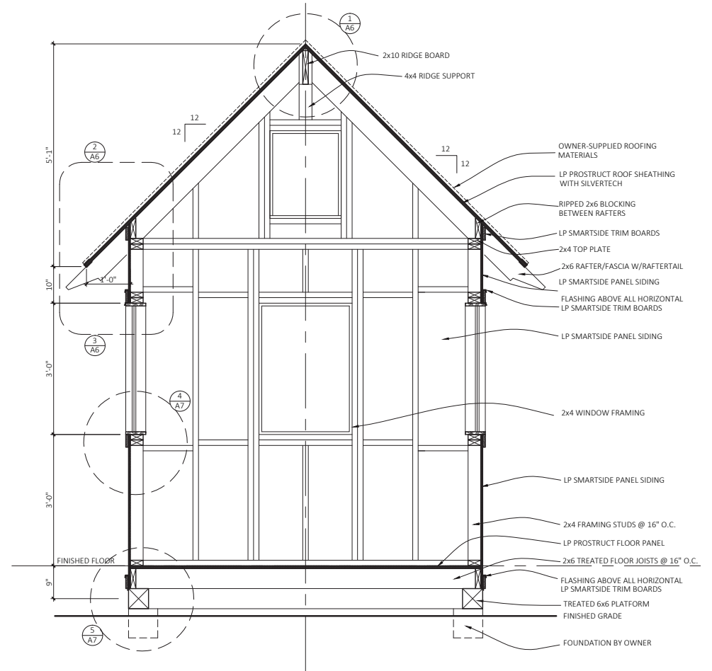
Cross-Section
