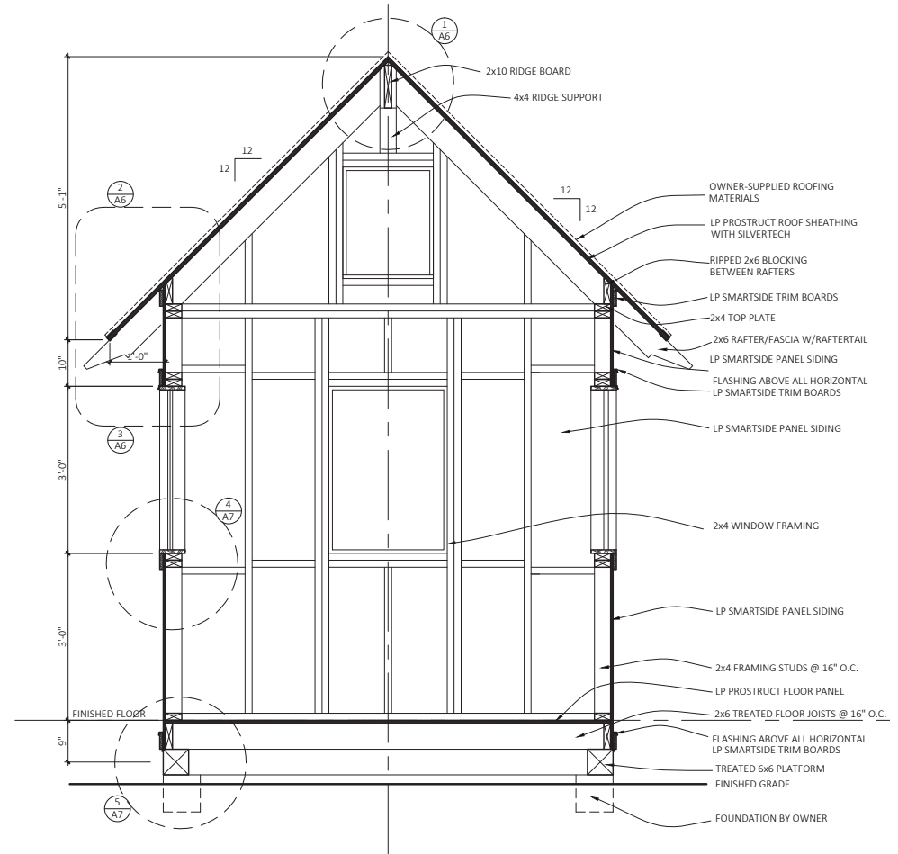
Cross-Section
