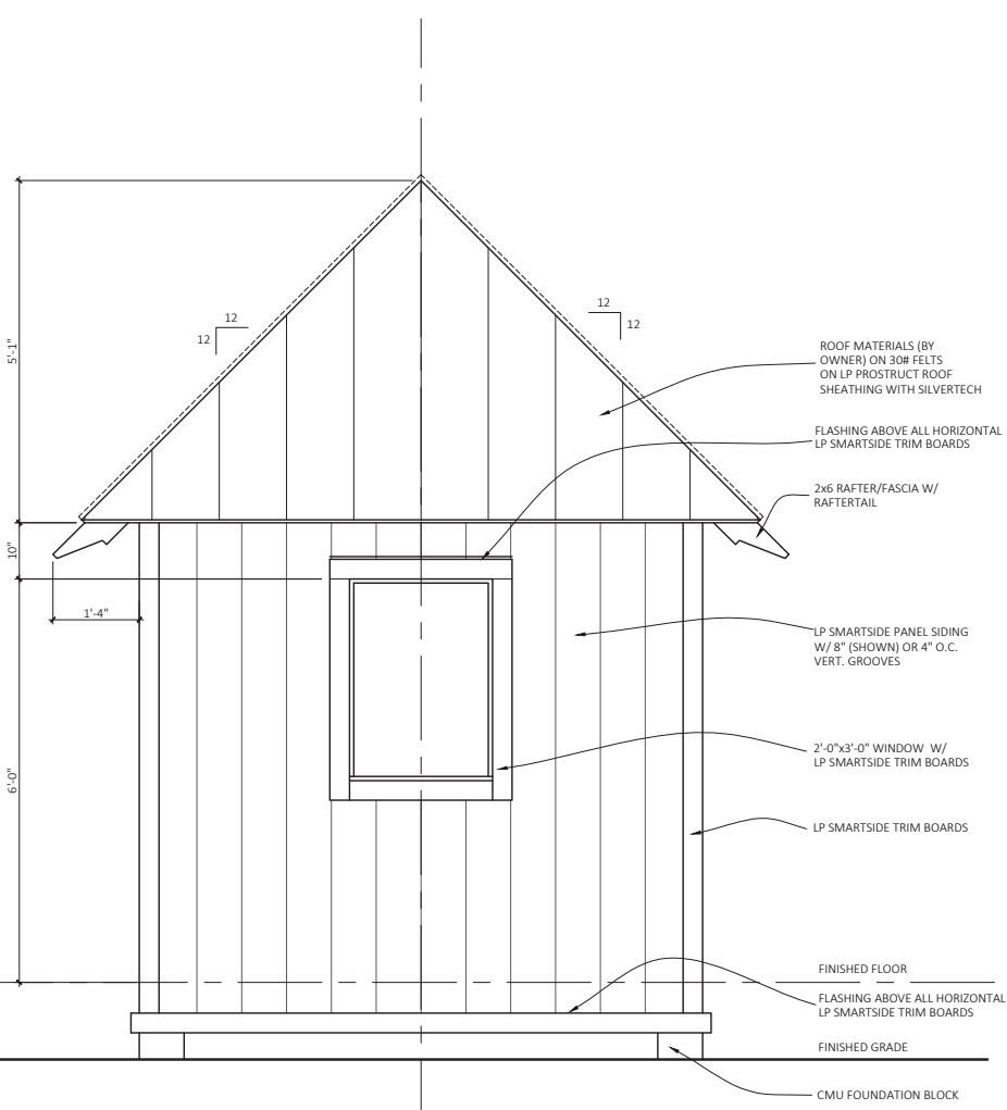
Rear Elevation
