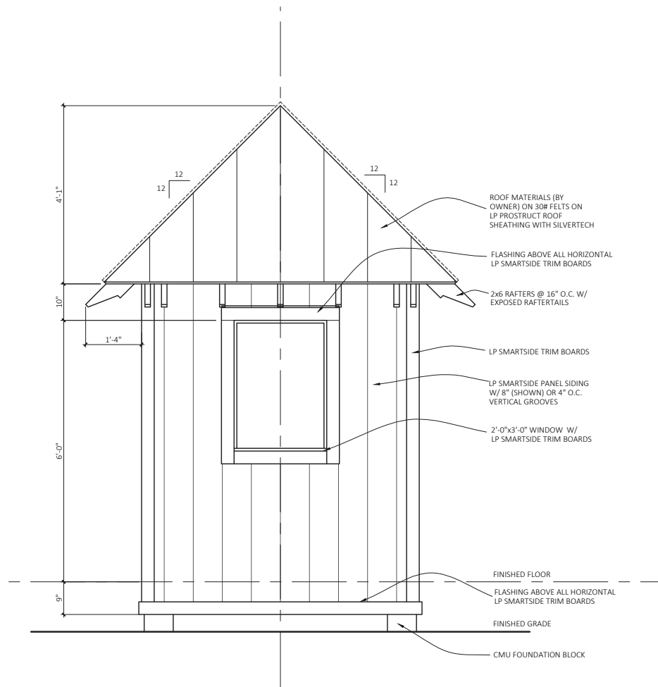
Rear Elevation
