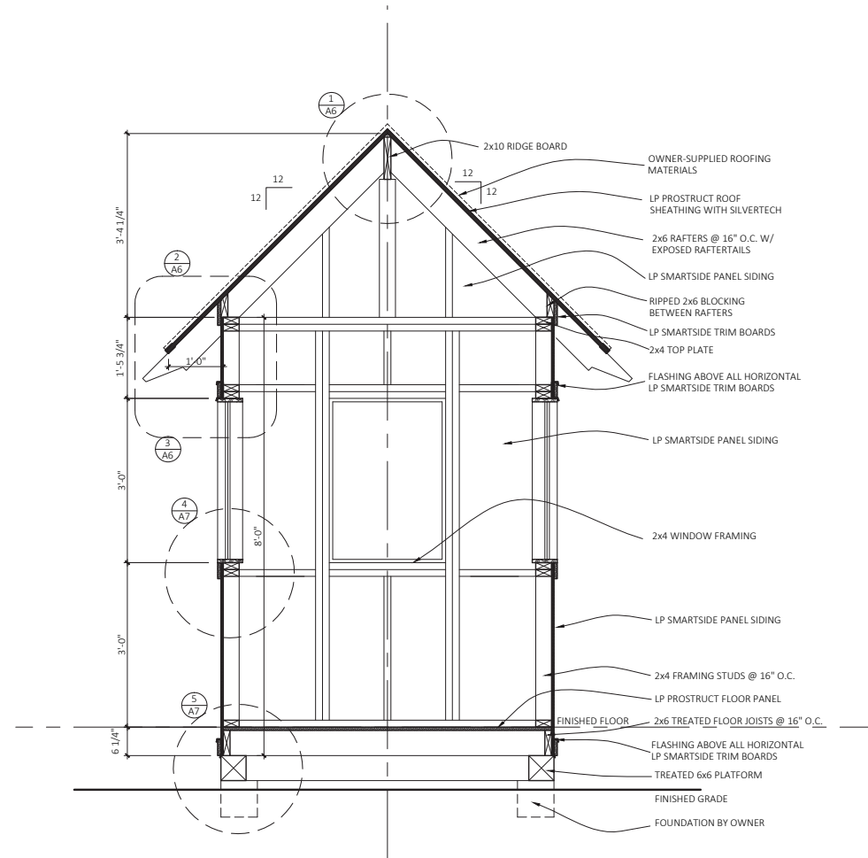
Cross-Section
