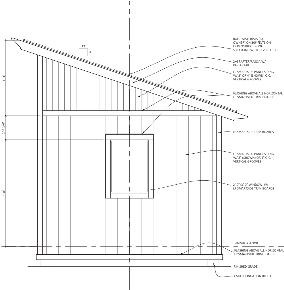
Rear Elevation
