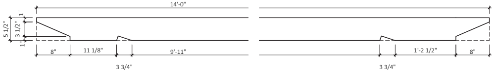
5 Roof Rafter Cuts
