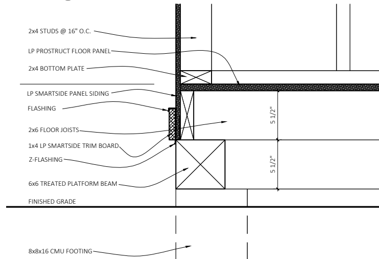
4 Detail
