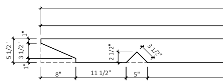
5 Roof Rafter Cuts
