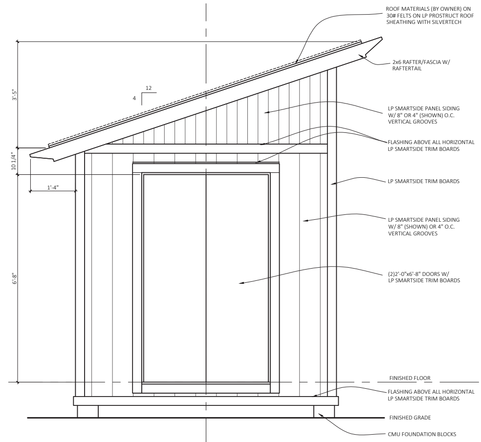
Front Elevation
