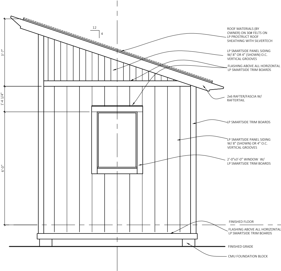
Rear Elevation
