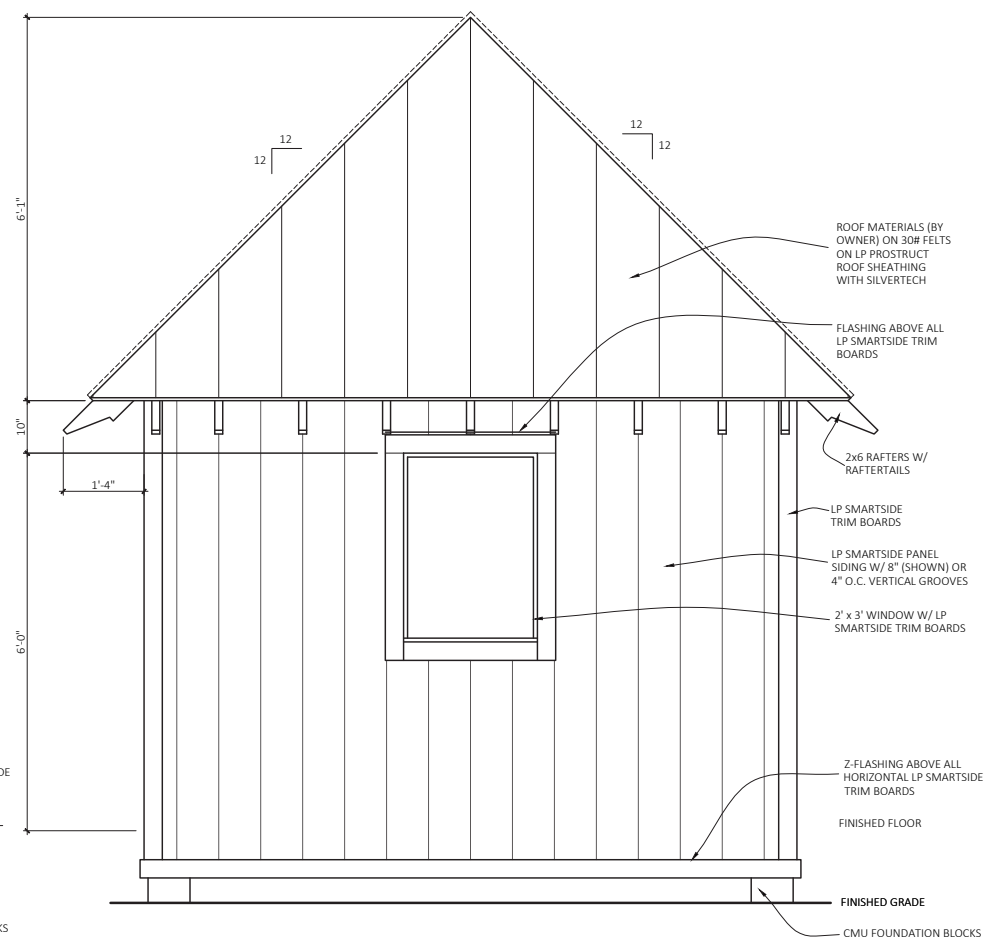
Rear Elevation
