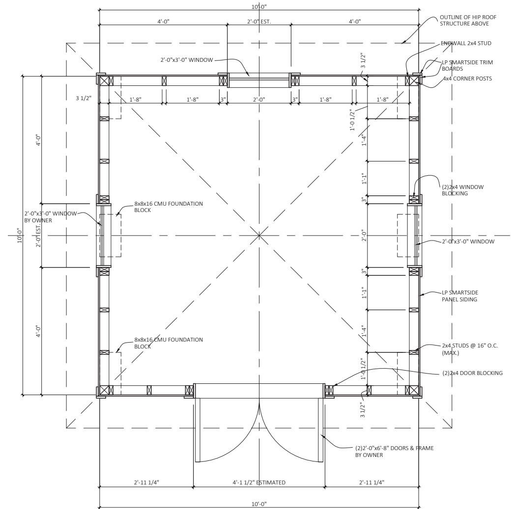
Floor Plan
